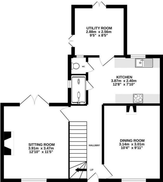
GROUND FLOOR 49.6 sq.m. (534 sq.ft.) approx.
